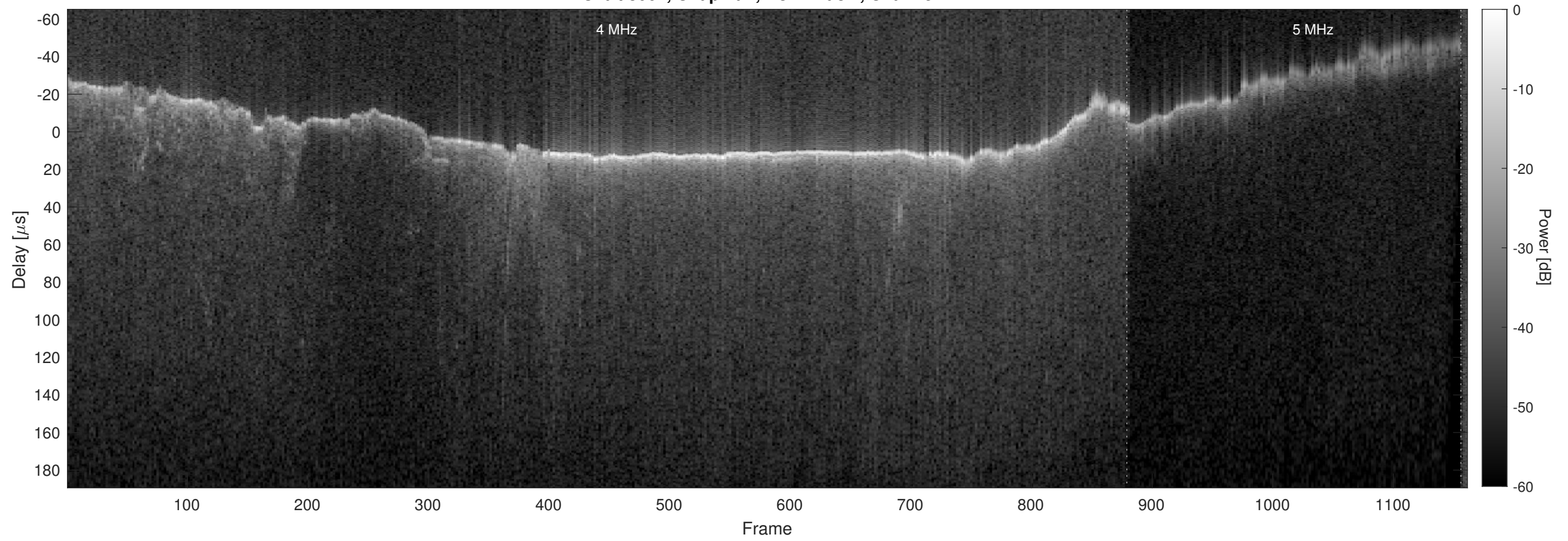
Orbit 8062, Chapman, No Window, Channel 2
