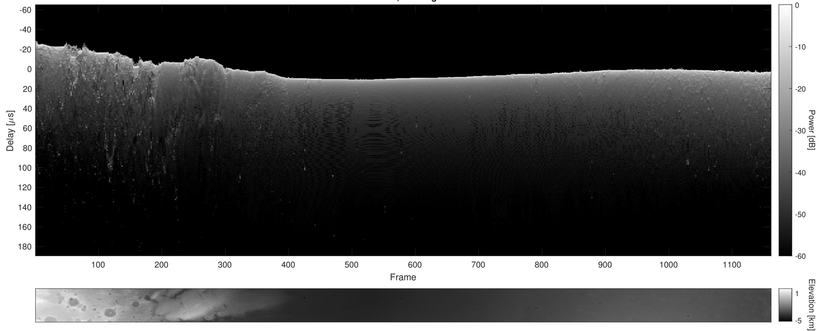
Orbit 8062, Cluttergram
