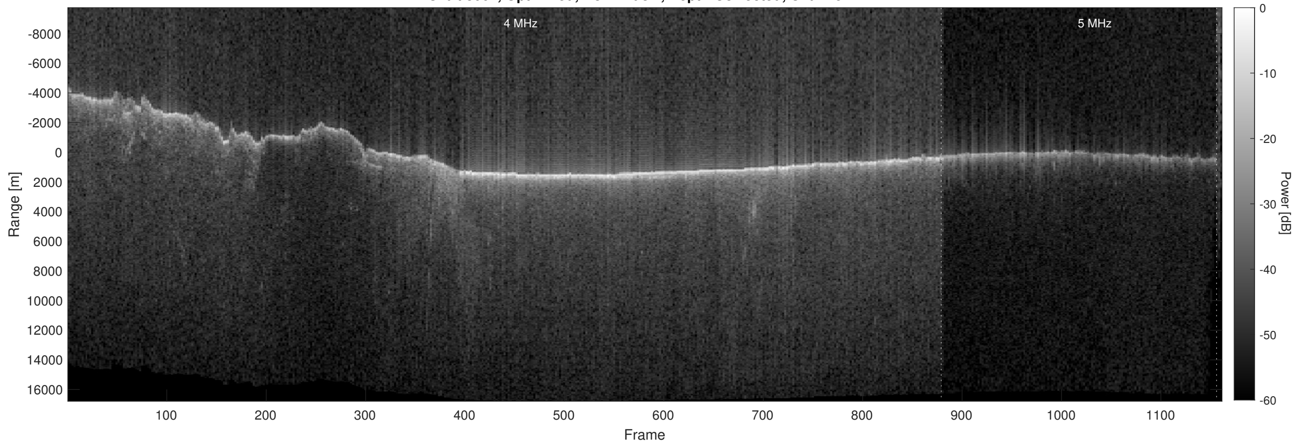
Orbit 8062, Optimized, No Window, Depth-Corrected, Channel 2
