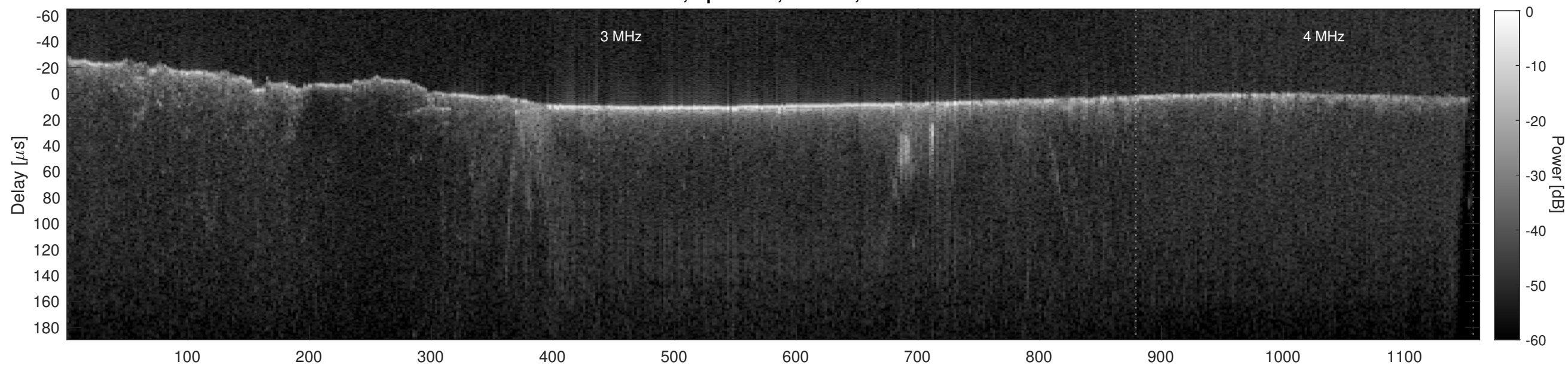
Orbit 8062, Cluttergram
