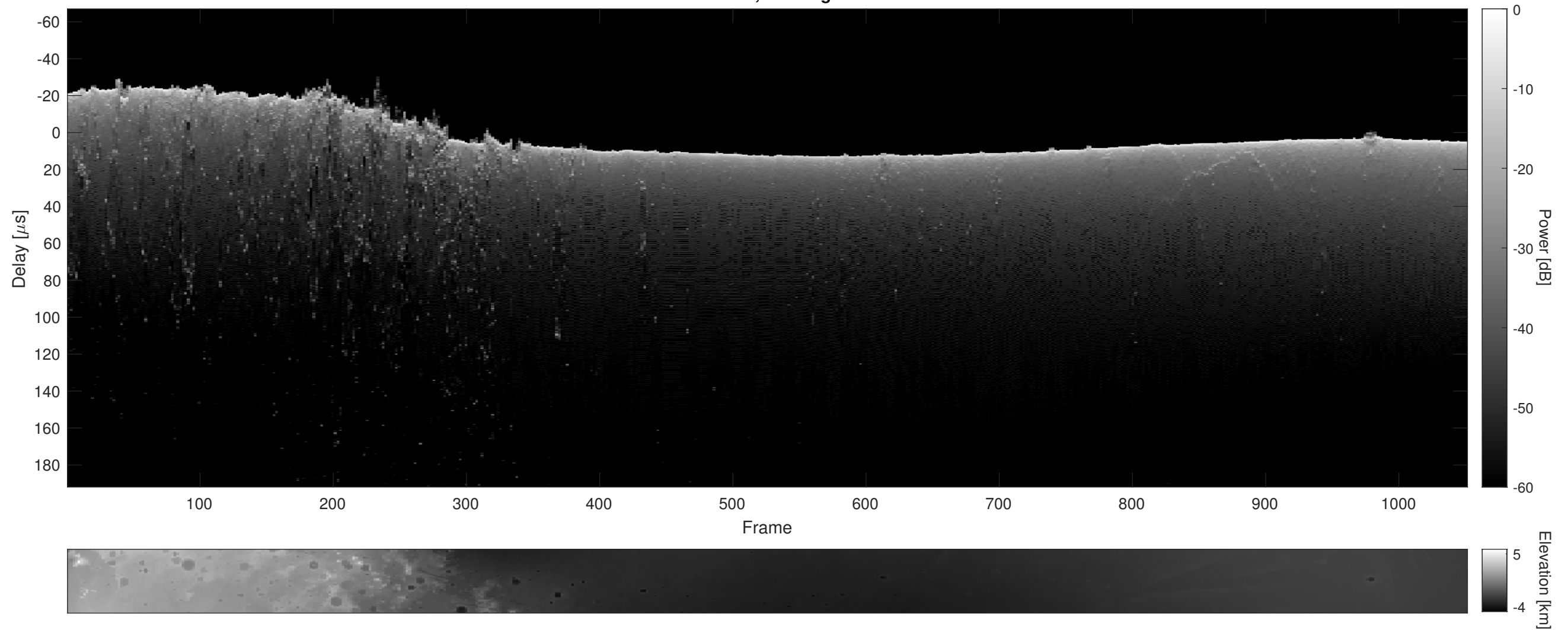
Orbit 8063, Cluttergram
