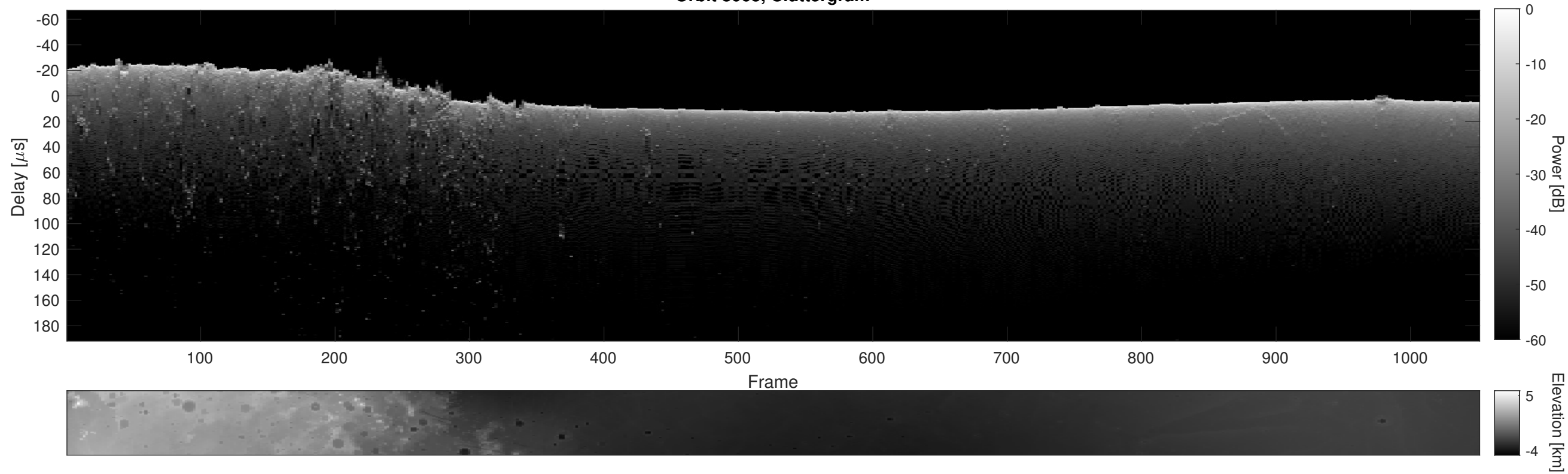
Orbit 8063, Cluttergram
