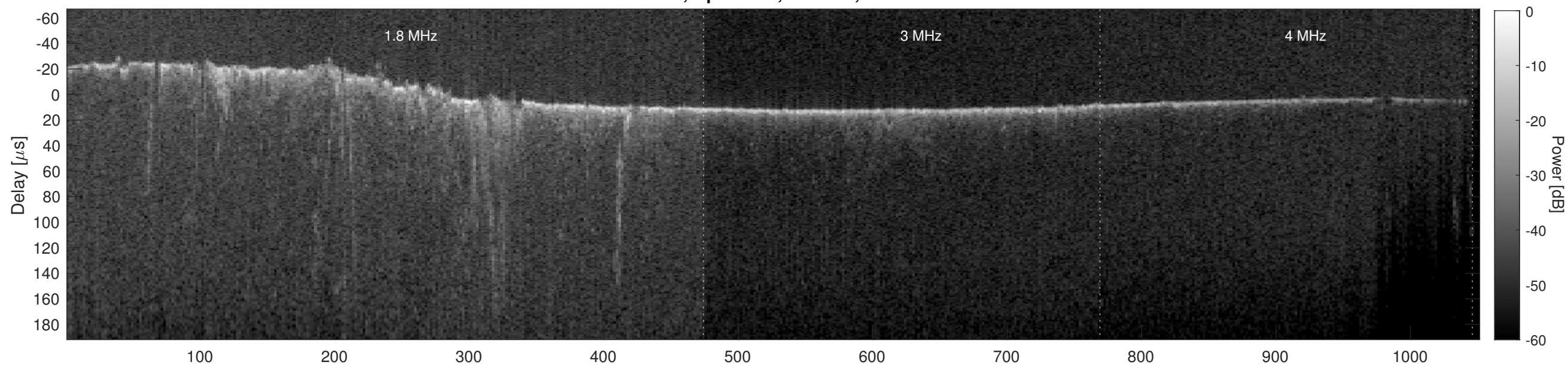
Orbit 8063, Cluttergram
