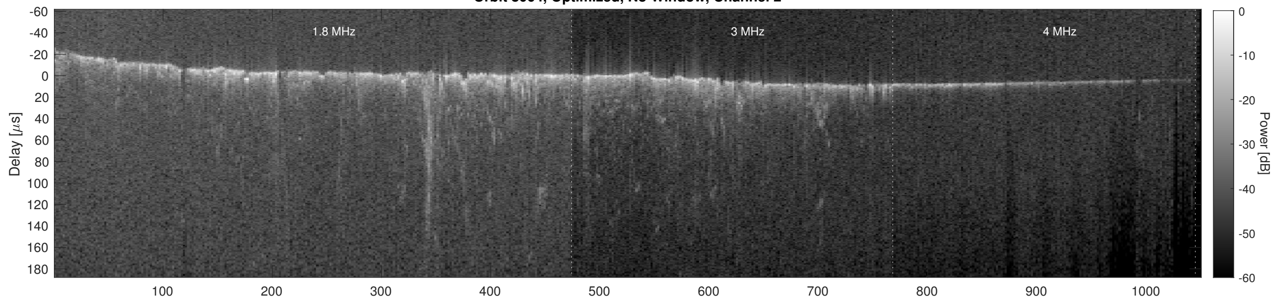
Orbit 8064, Cluttergram
