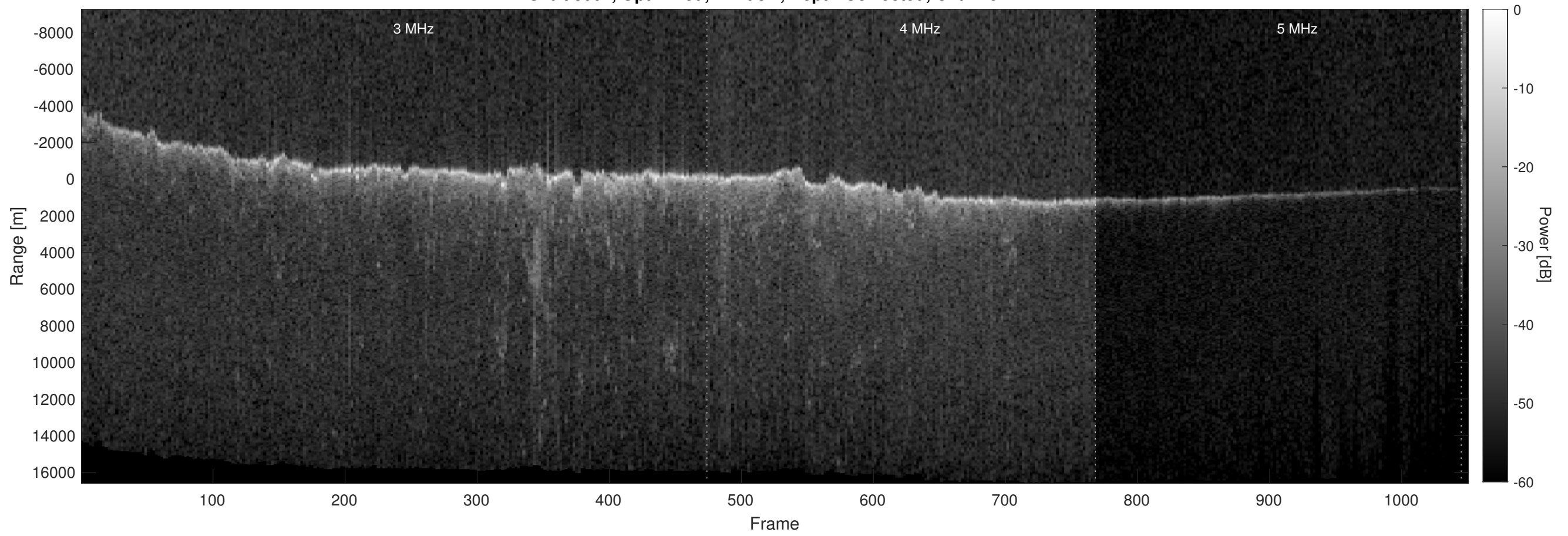
Orbit 8064, Optimized, Window, Depth-Corrected, Channel 2
