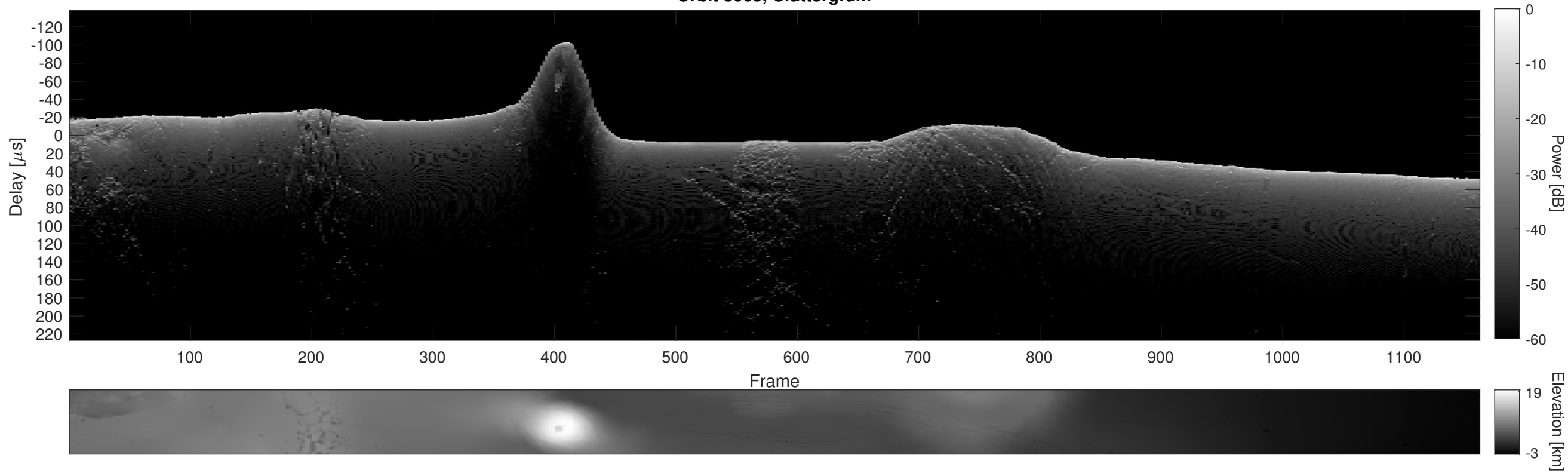
Orbit 8065, Cluttergram
