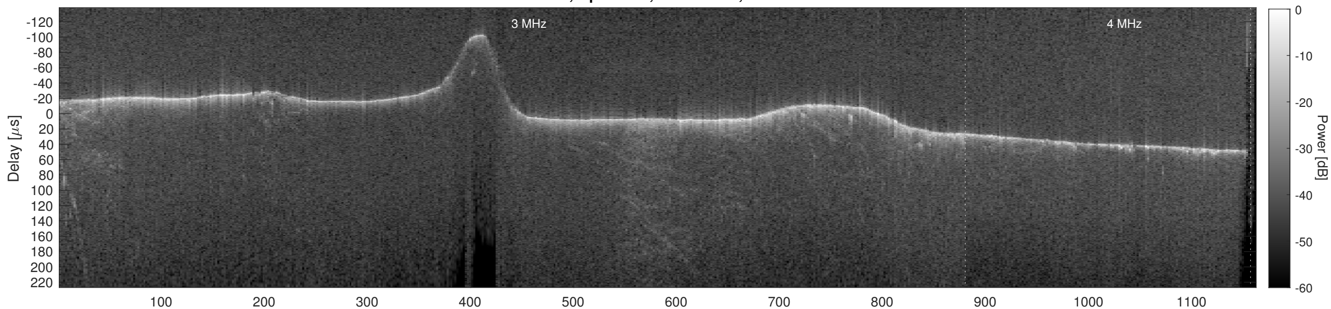
Orbit 8065, Cluttergram
