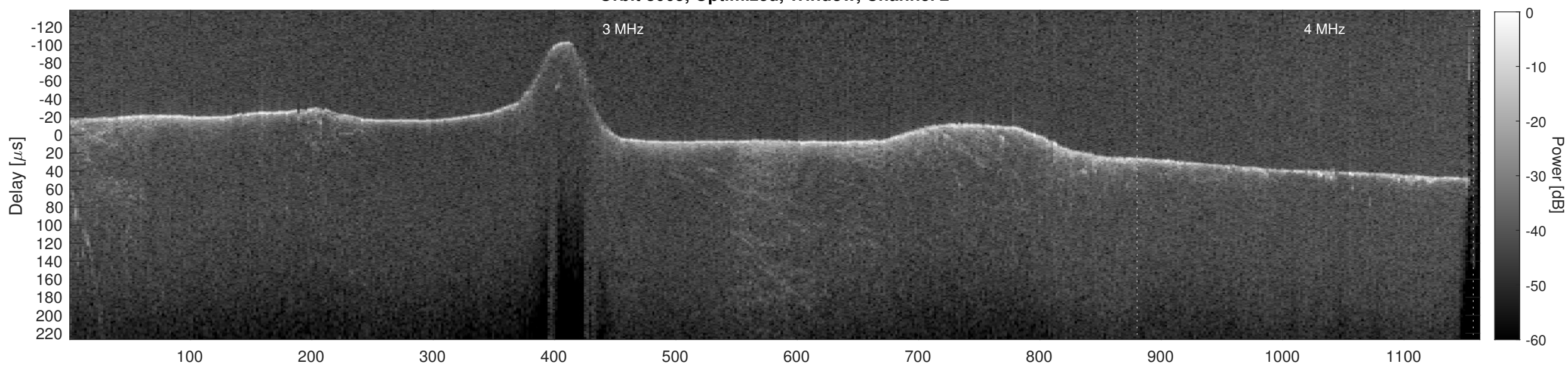
Orbit 8065, Cluttergram
