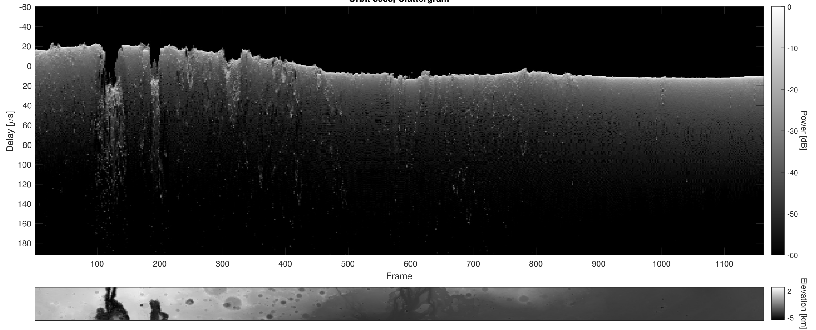
Orbit 8068, Cluttergram
