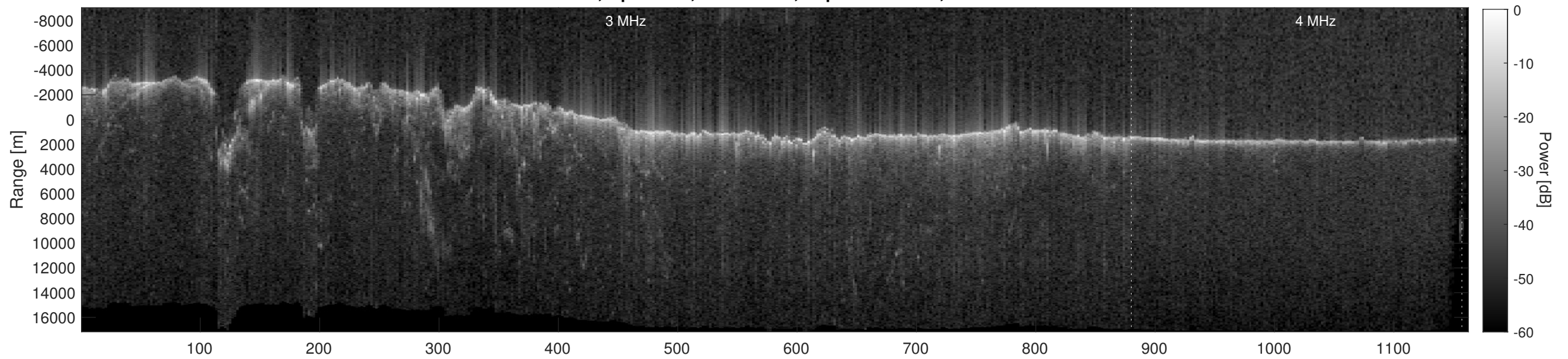
Orbit 8068, Depth-Corrected Cluttergram
