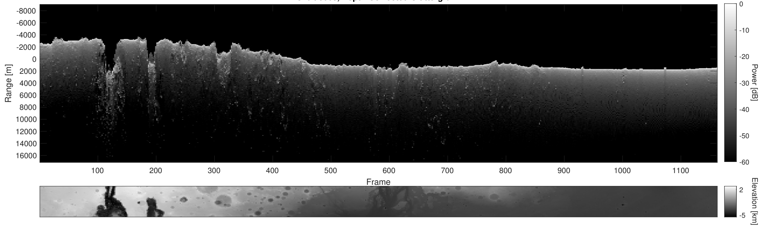
Orbit 8068, Depth-Corrected Cluttergram
