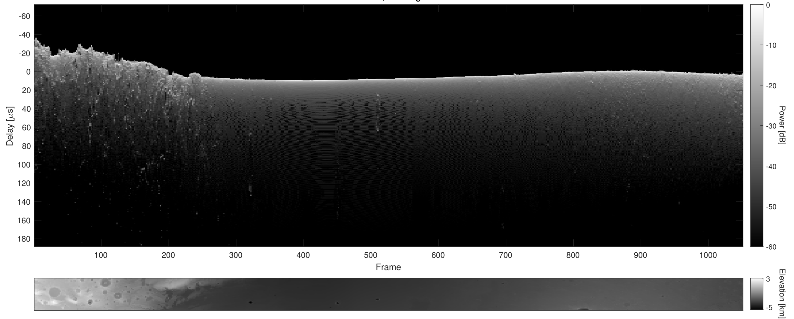
Orbit 8069, Cluttergram
