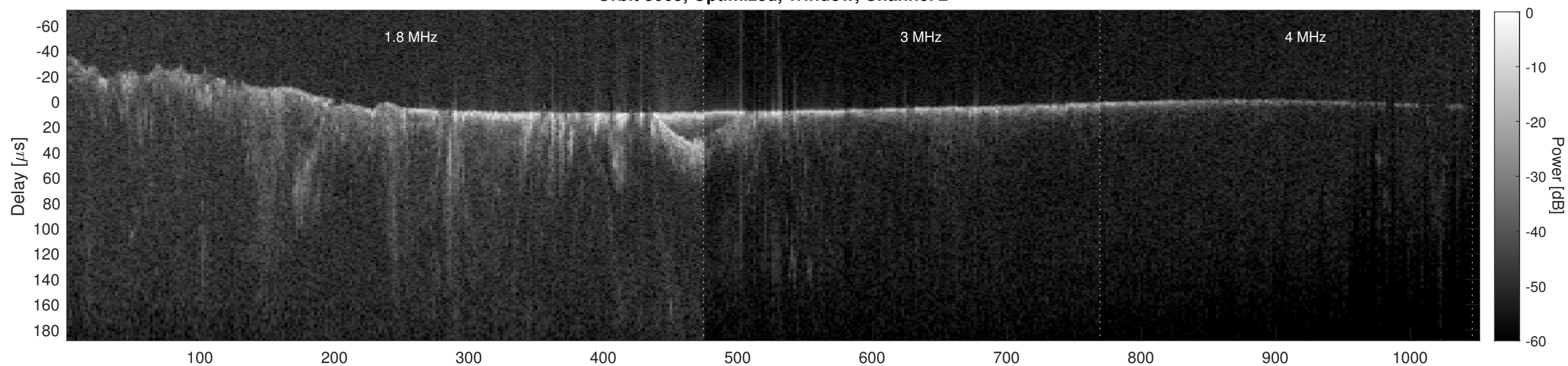
Orbit 8069, Cluttergram
