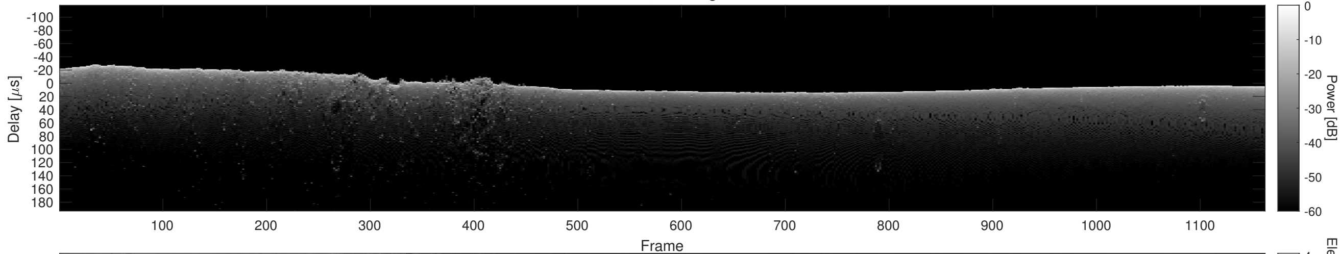
Orbit 8070, Cluttergram
