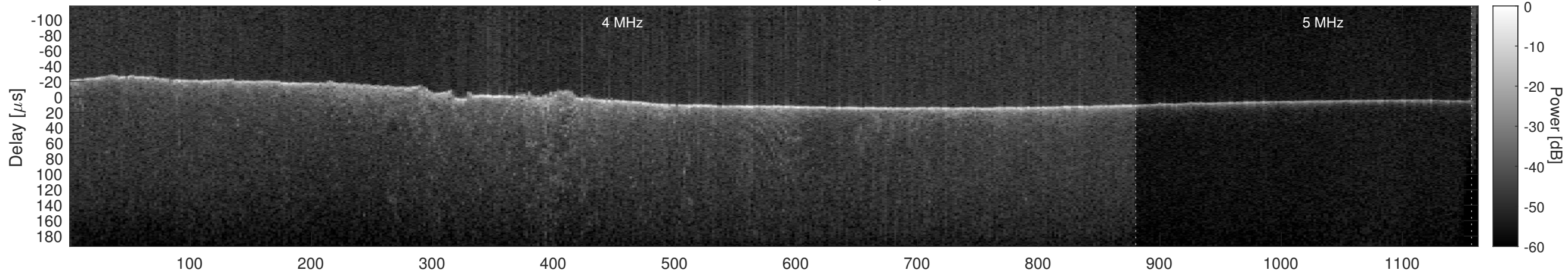
Orbit 8070, Cluttergram
