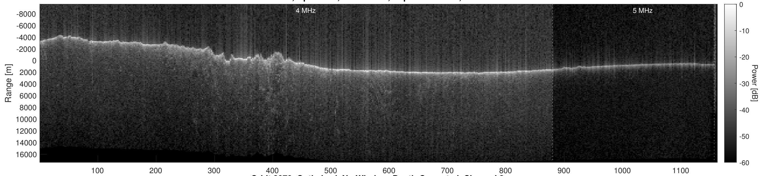
Orbit 8070, Optimized, No Window, Depth-Corrected, Channel 2
