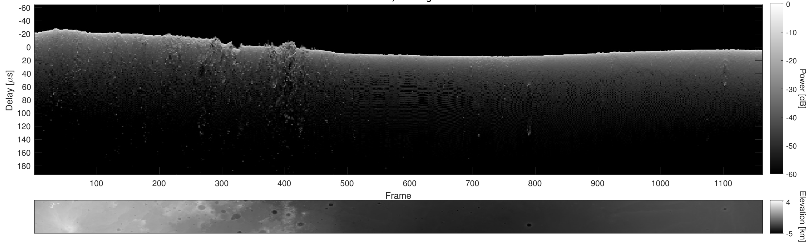
Orbit 8070, Cluttergram
