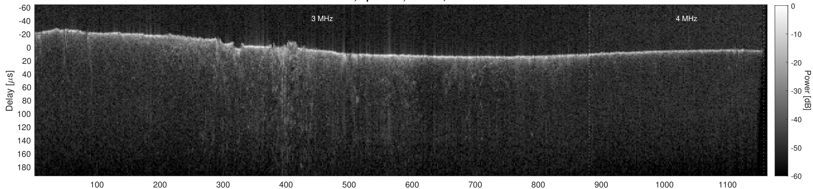
Orbit 8070, Cluttergram
