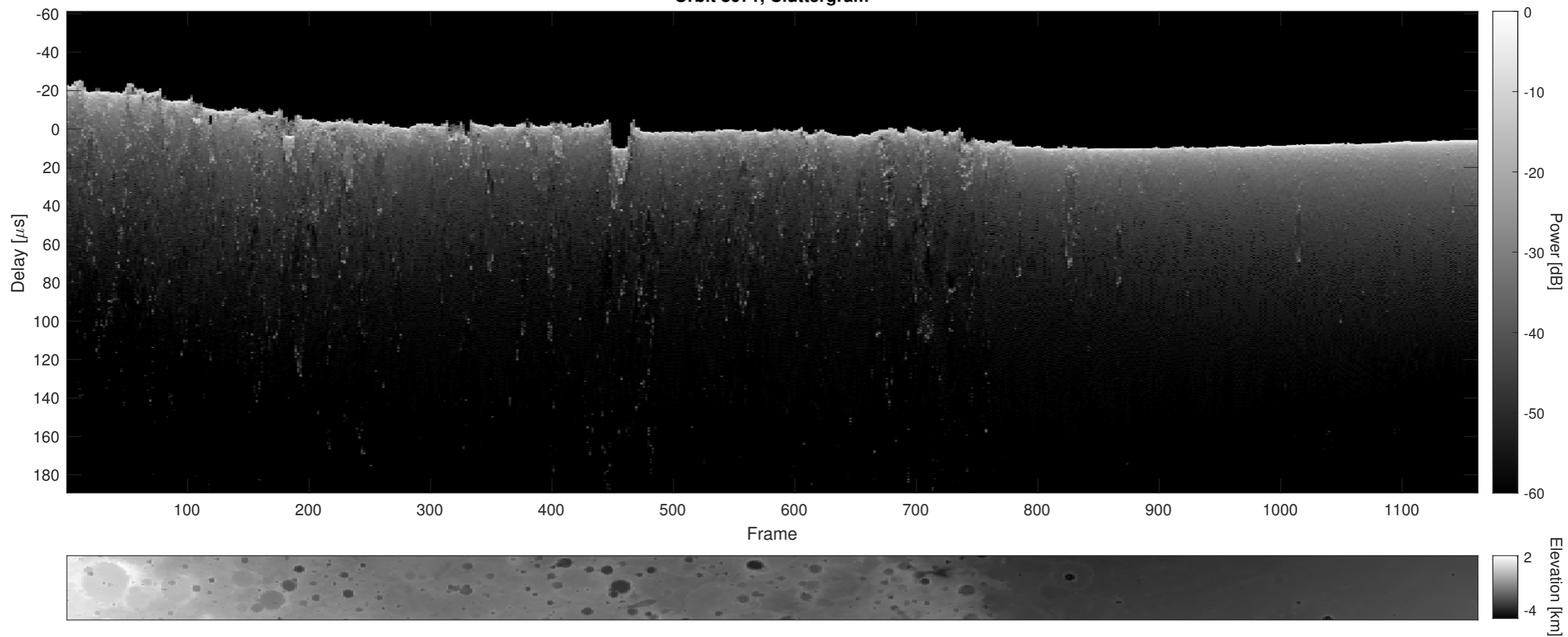
Orbit 8071, Cluttergram
