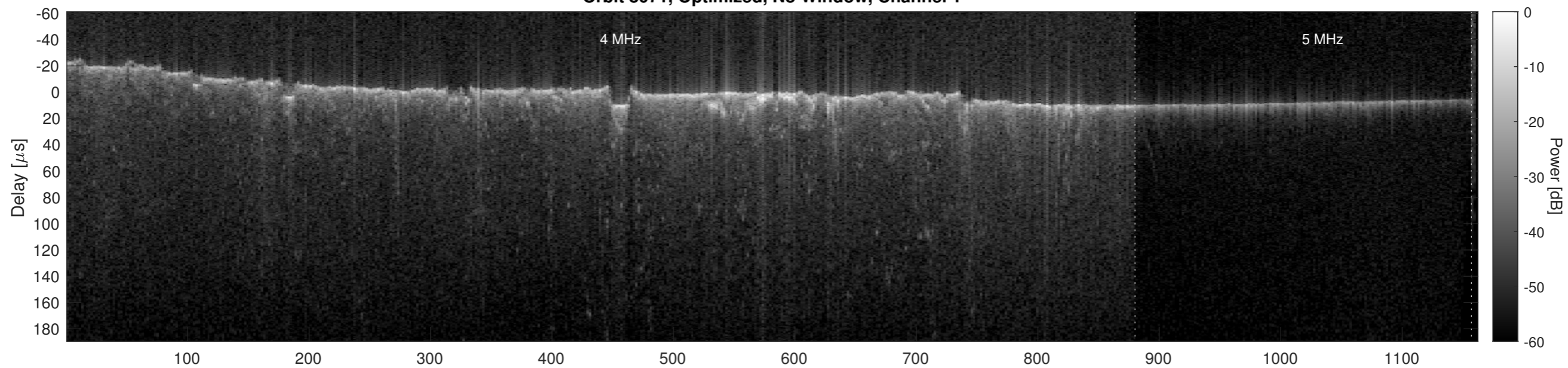
Orbit 8071, Optimized, No Window, Channel 2
