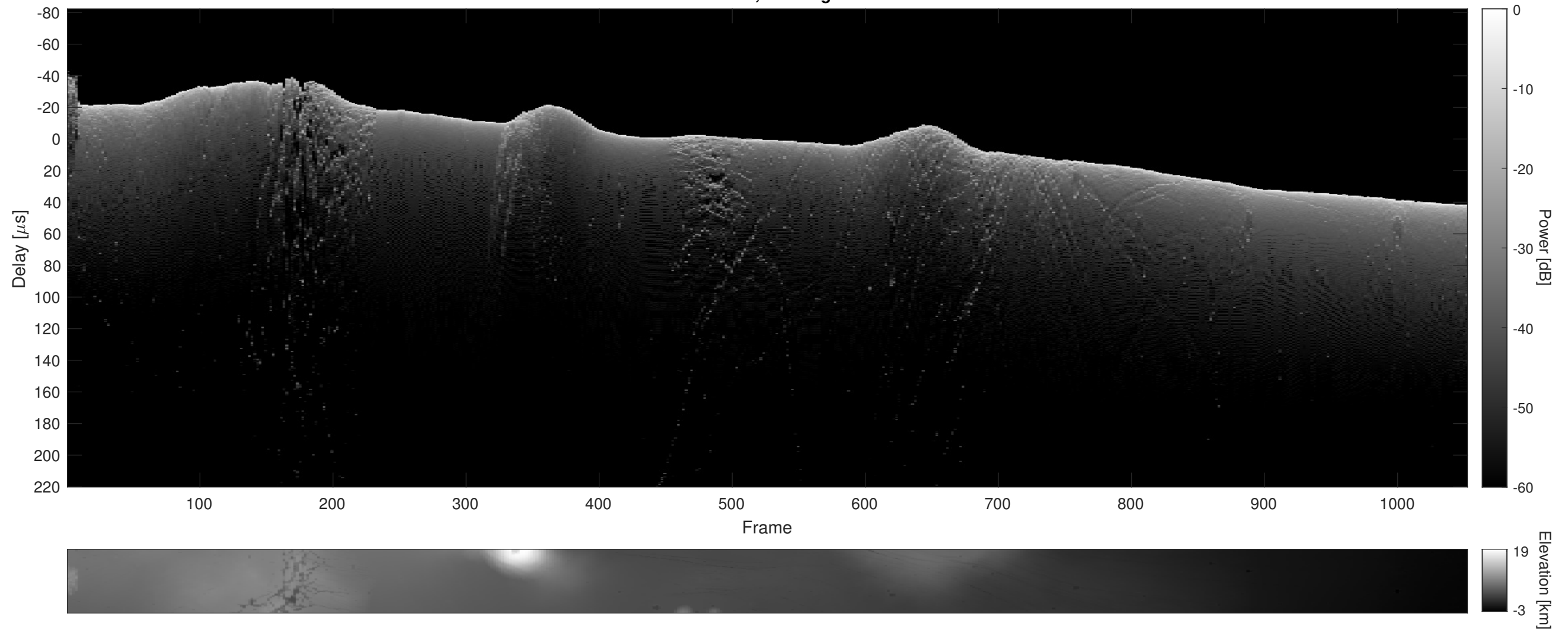
Orbit 8072, Cluttergram
