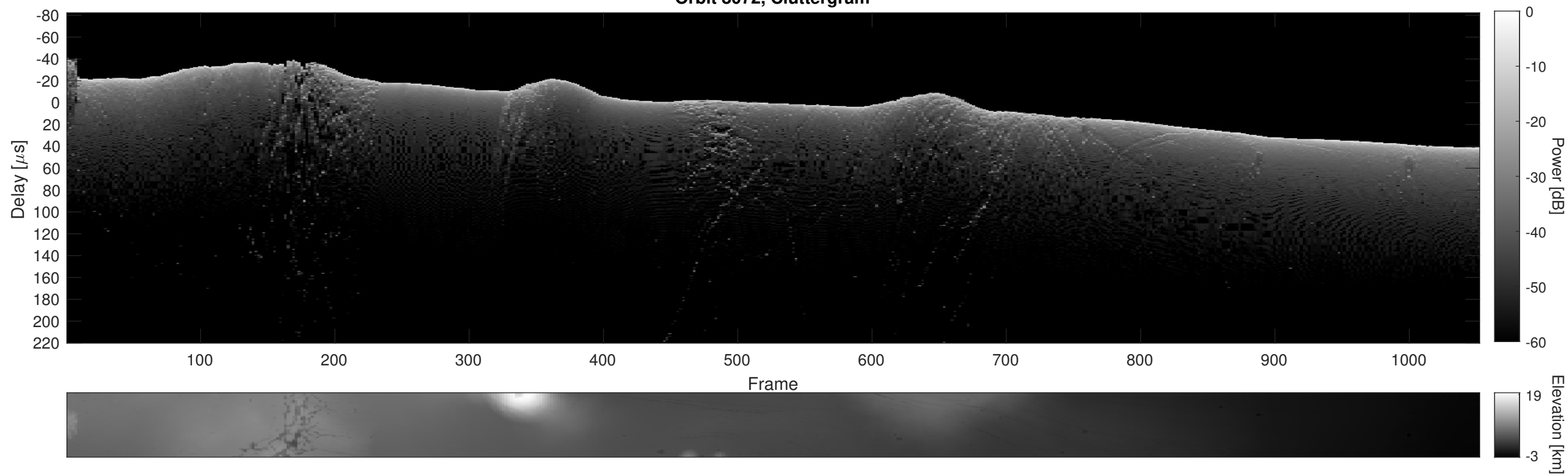
Orbit 8072, Cluttergram
