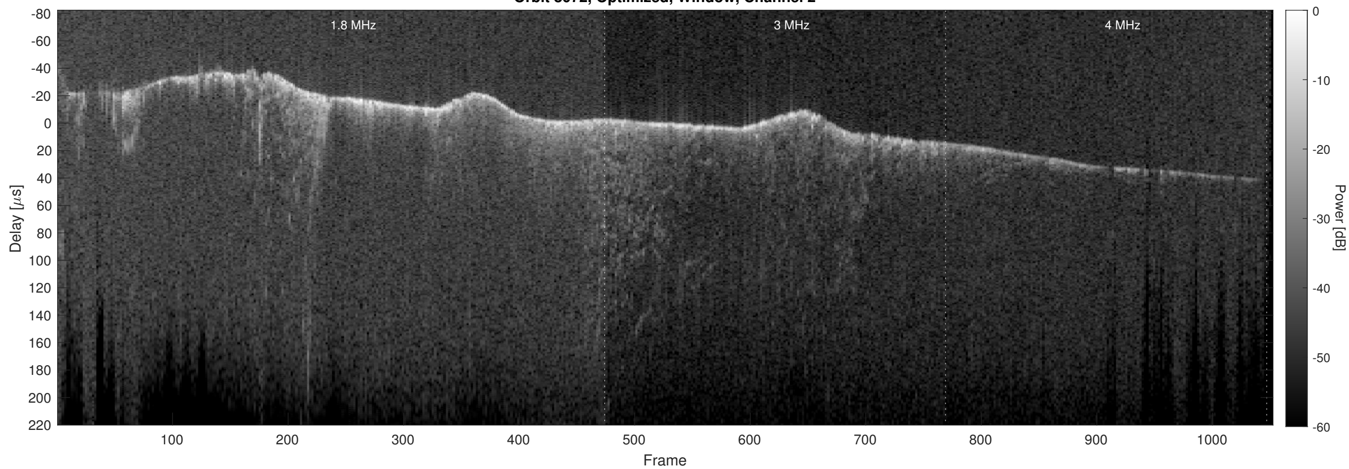
Orbit 8072, Optimized, Window, Channel 2
