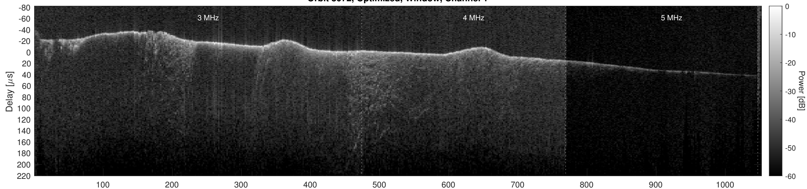
Orbit 8072, Optimized, Window, Channel 2
