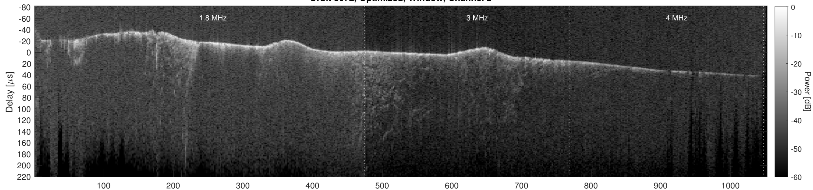
Orbit 8072, Cluttergram
