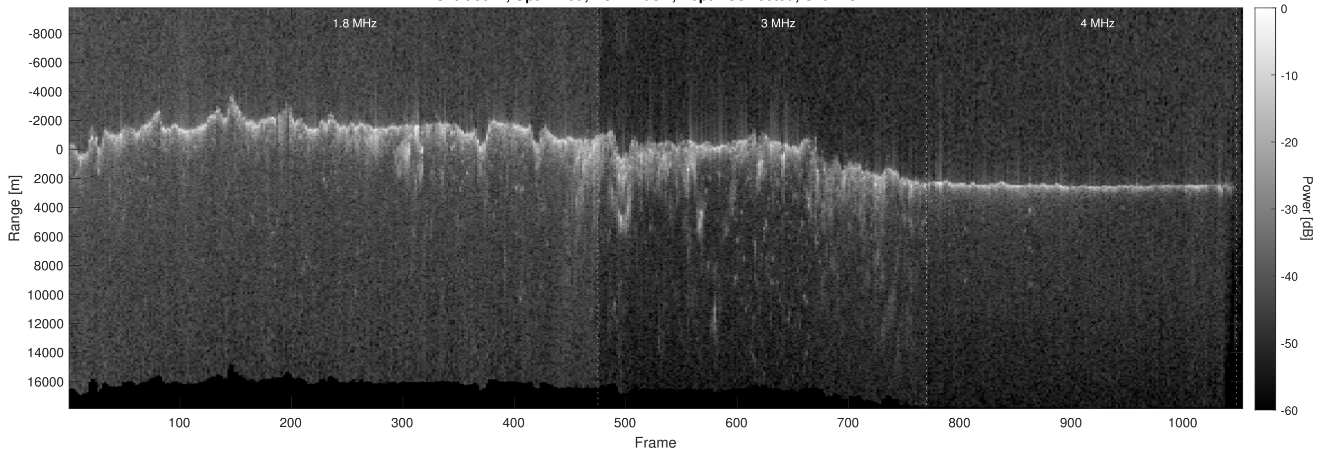
Orbit 8074, Optimized, No Window, Depth-Corrected, Channel 2
