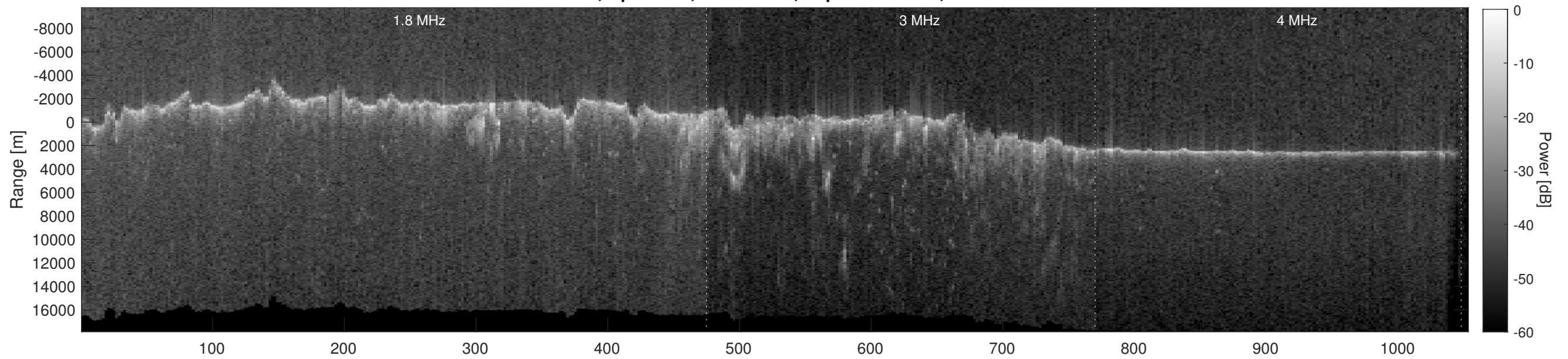
Orbit 8074, Depth-Corrected Cluttergram
