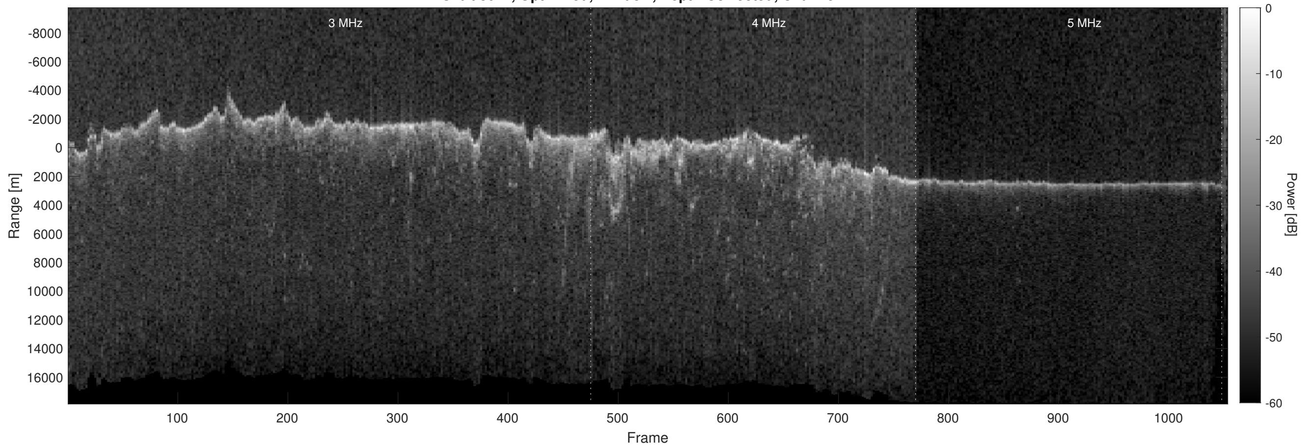
Orbit 8074, Optimized, Window, Depth-Corrected, Channel 2
