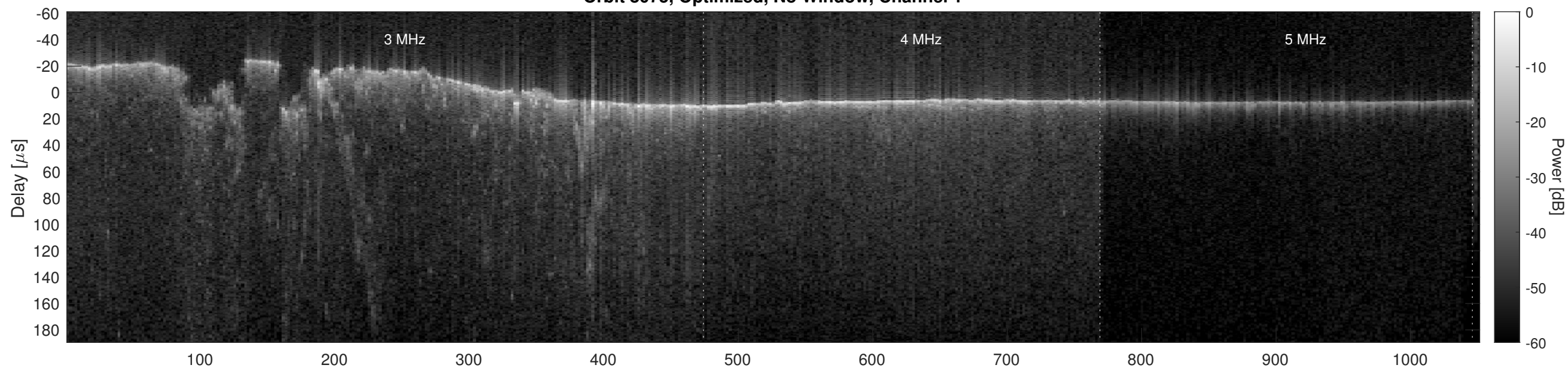
Orbit 8075, Optimized, No Window, Channel 2
