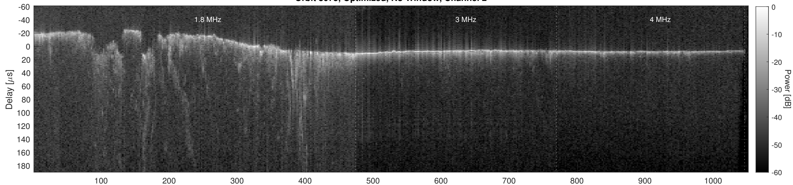
Orbit 8075, Cluttergram
