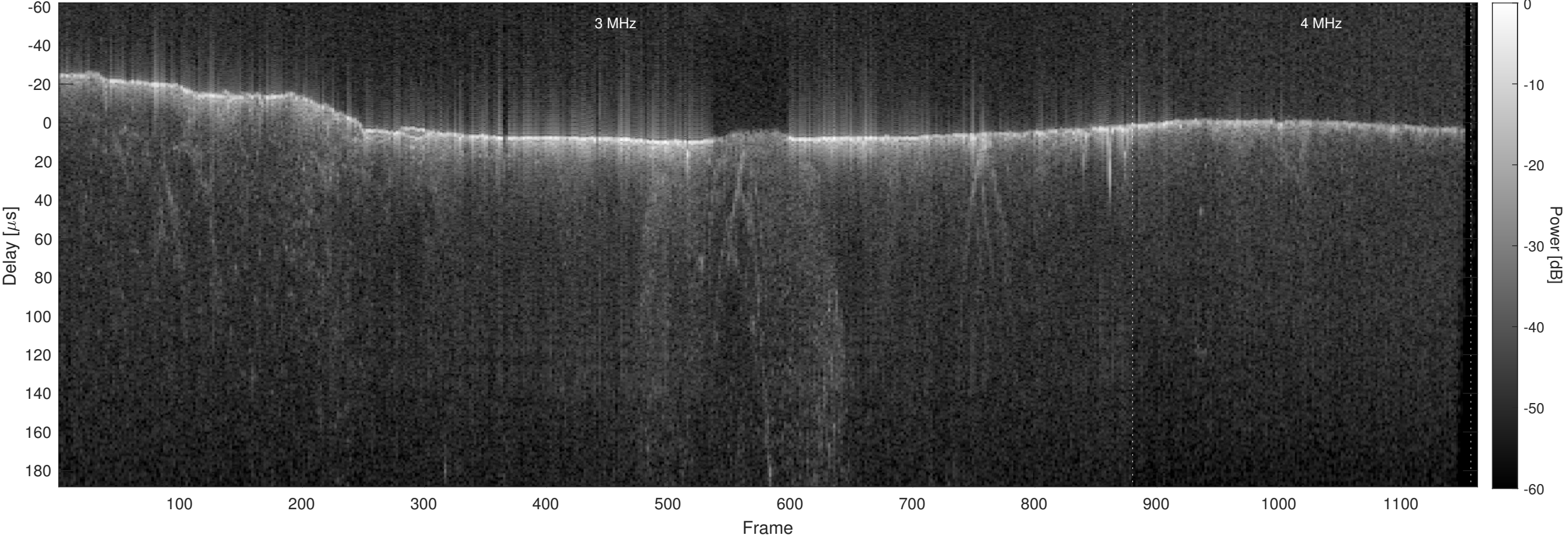
Orbit 8076, Optimized, No Window, Channel 2
