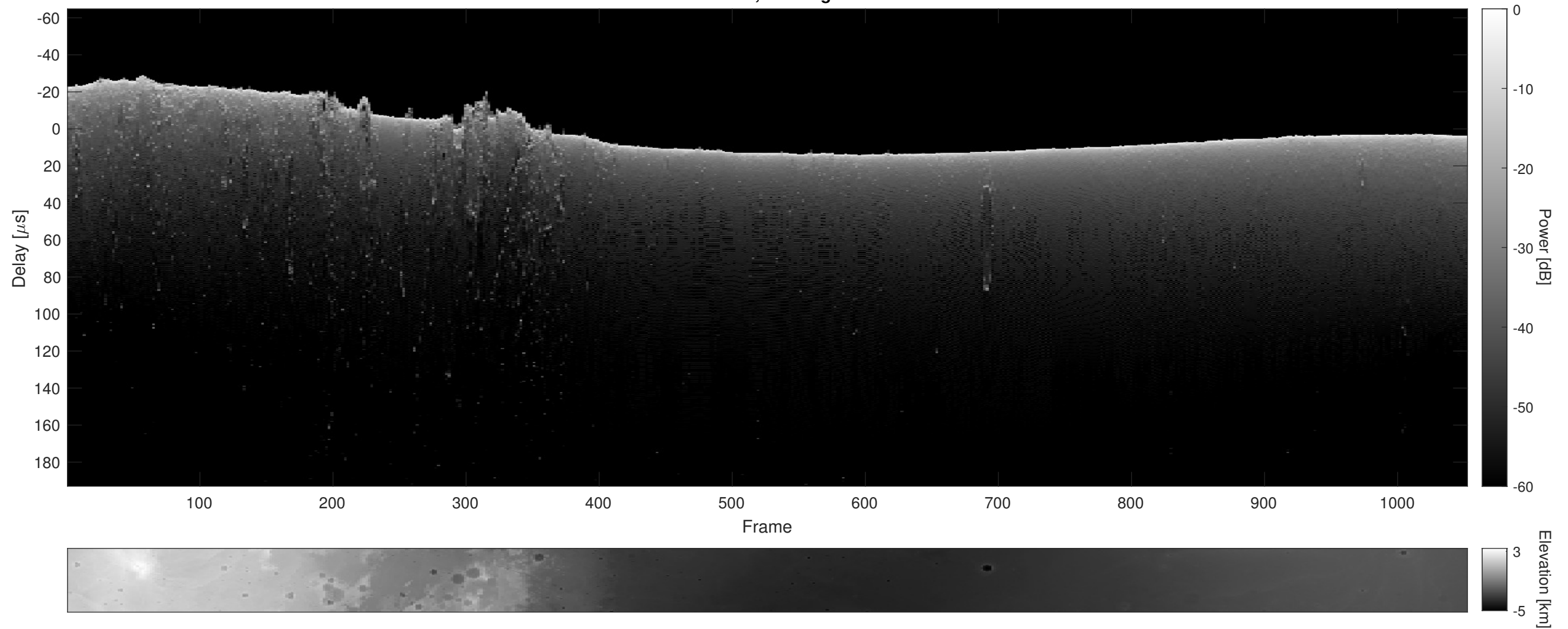
Orbit 8077, Cluttergram
