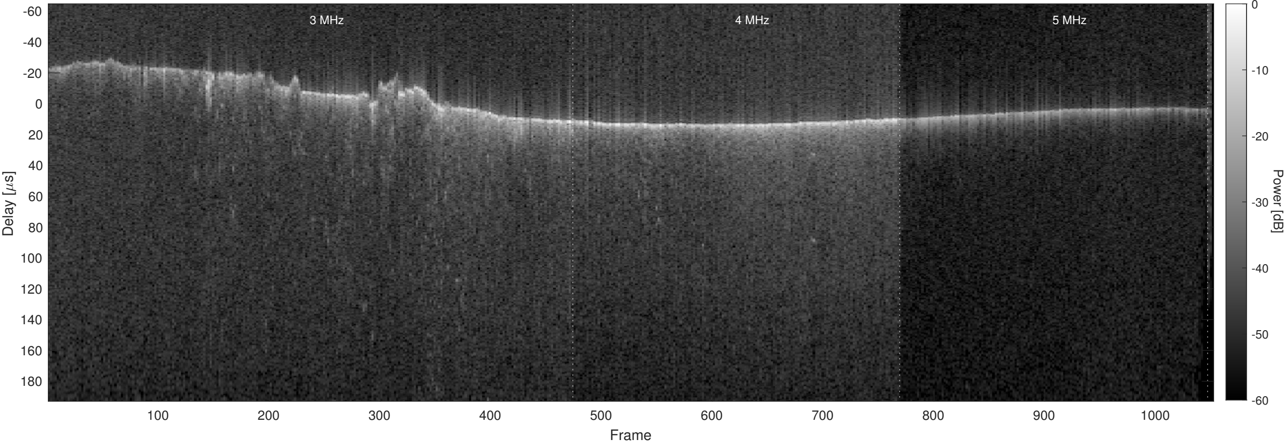
Orbit 8077, Optimized, No Window, Channel 2
