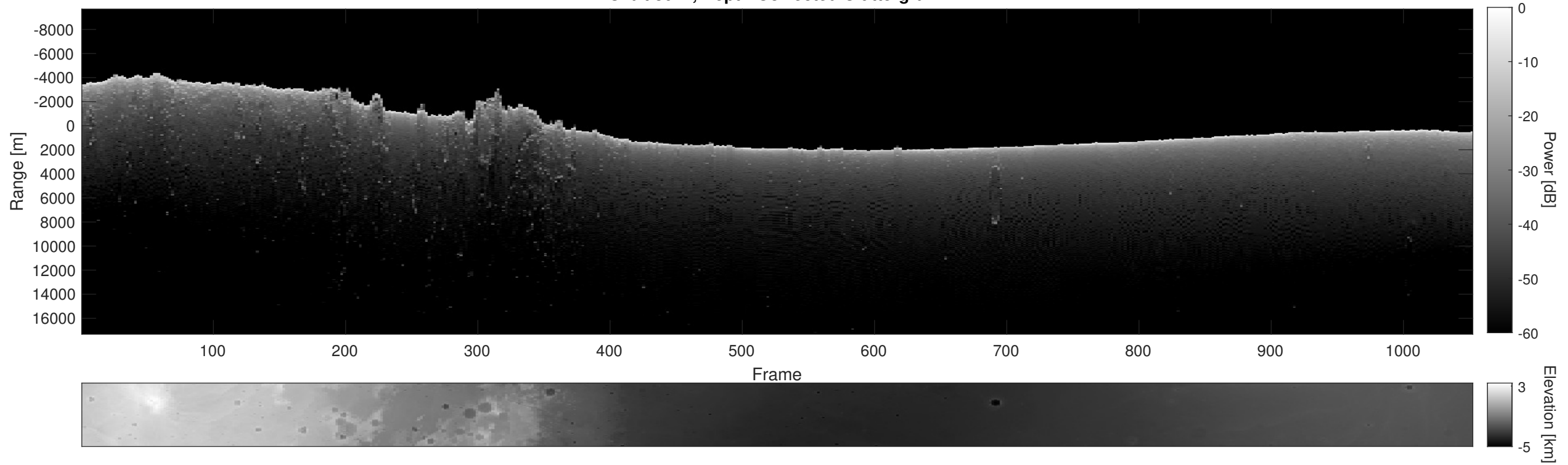
Orbit 8077, Depth-Corrected Cluttergram
