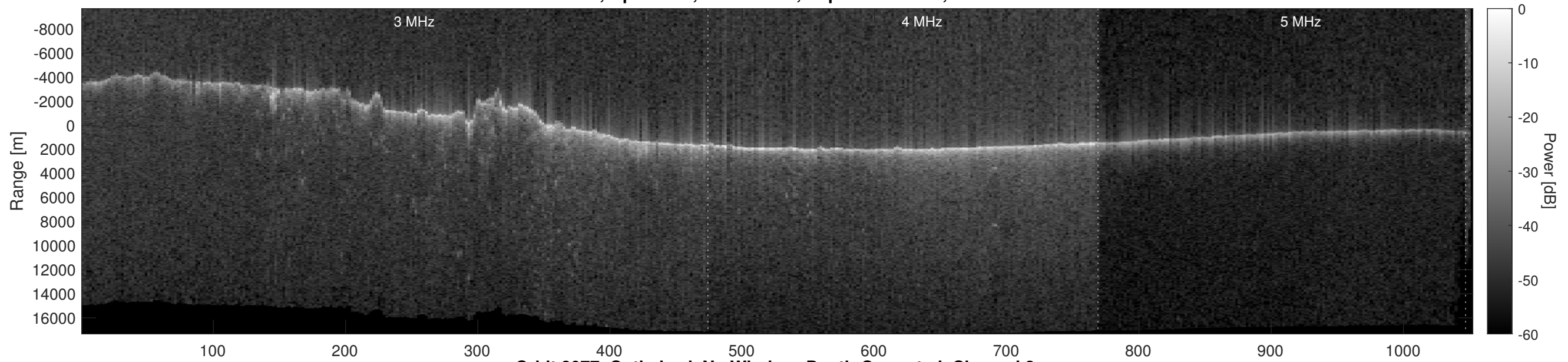
Orbit 8077, Optimized, No Window, Depth-Corrected, Channel 2
