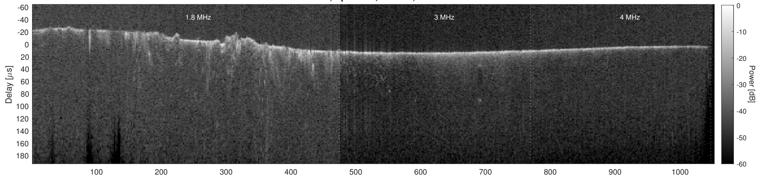
Orbit 8077, Cluttergram
