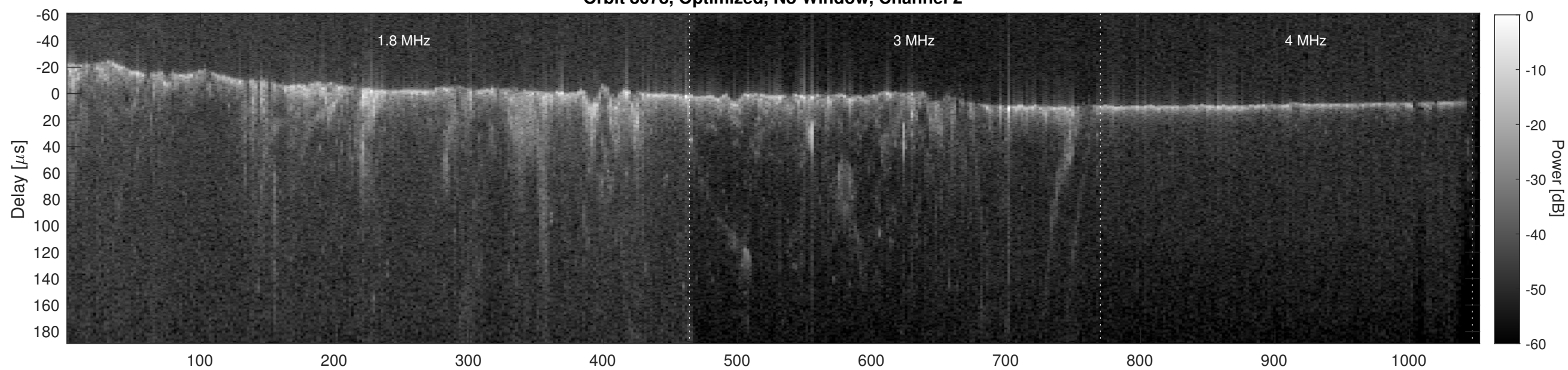
Orbit 8078, Cluttergram
