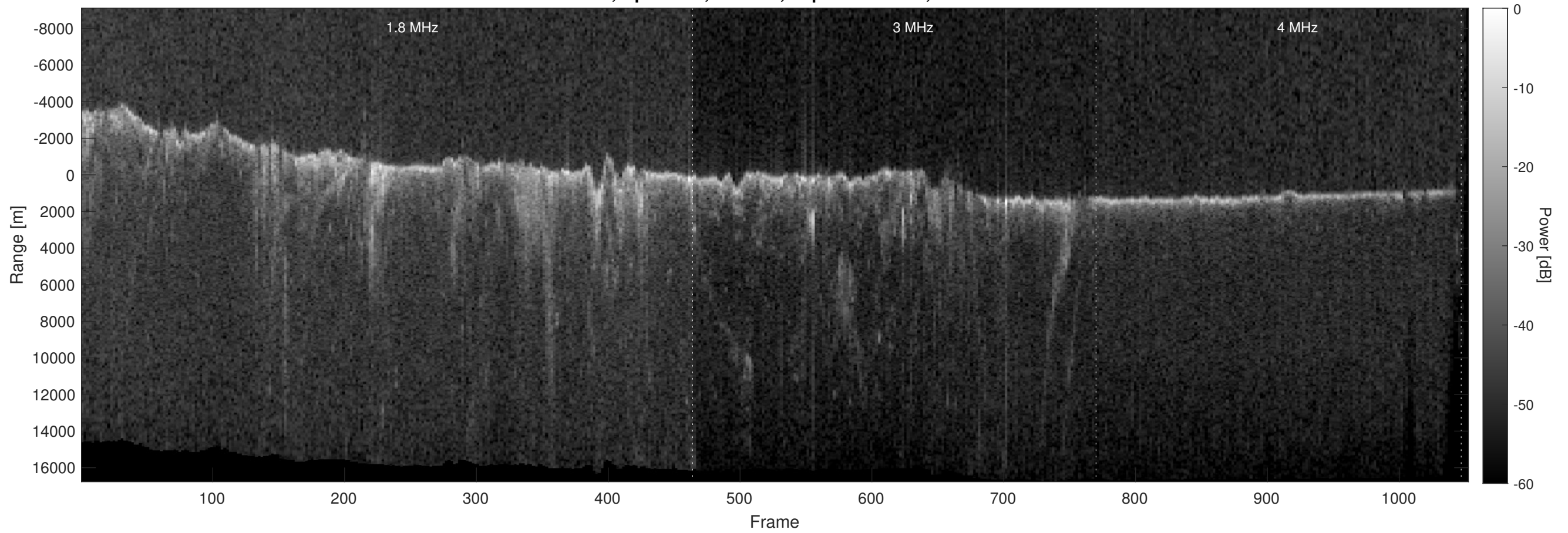
Orbit 8078, Optimized, Window, Depth-Corrected, Channel 2
