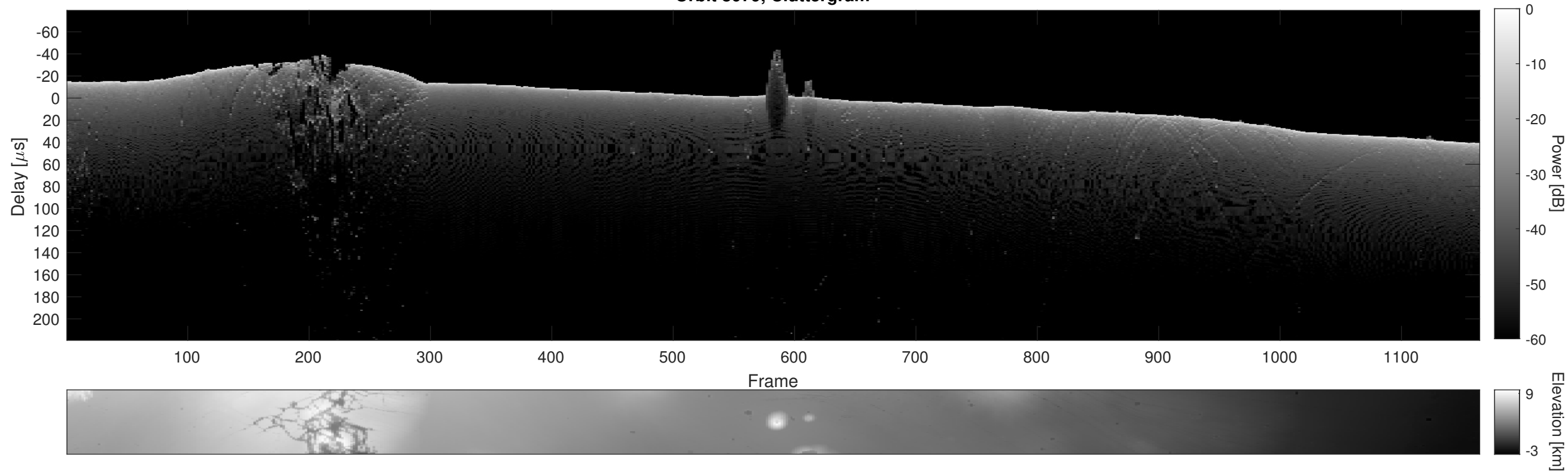
Orbit 8079, Cluttergram
