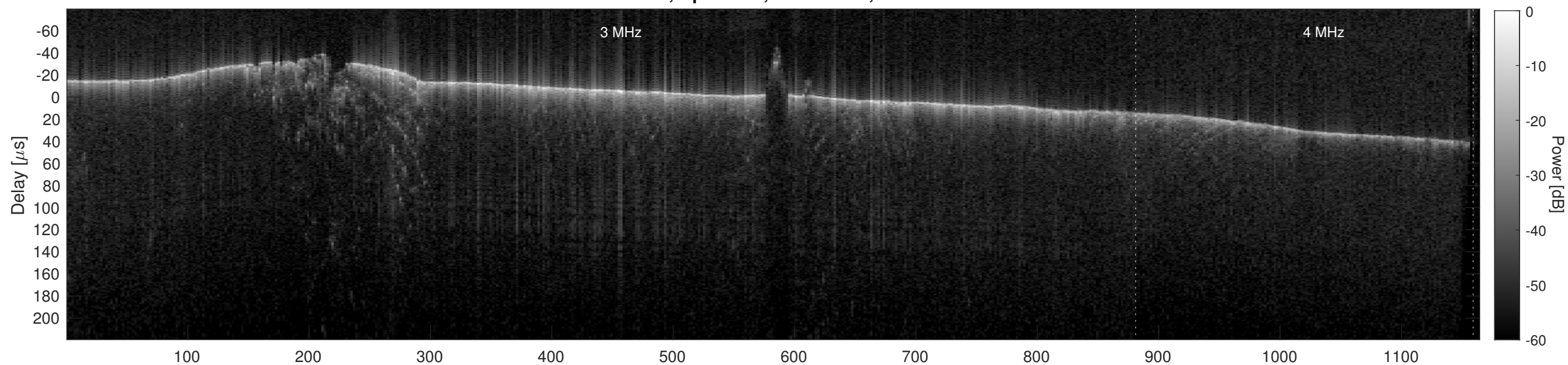
Orbit 8079, Cluttergram
