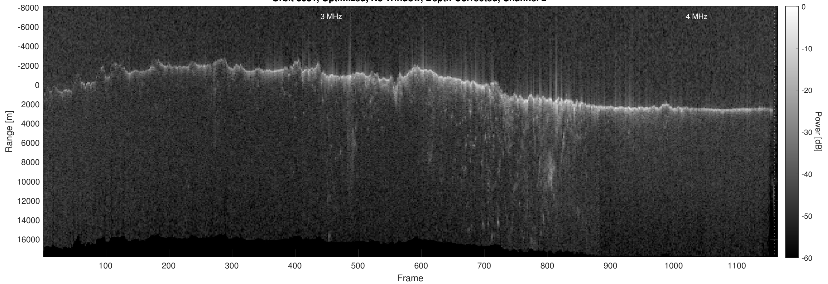
Orbit 8081, Optimized, No Window, Depth-Corrected, Channel 2
