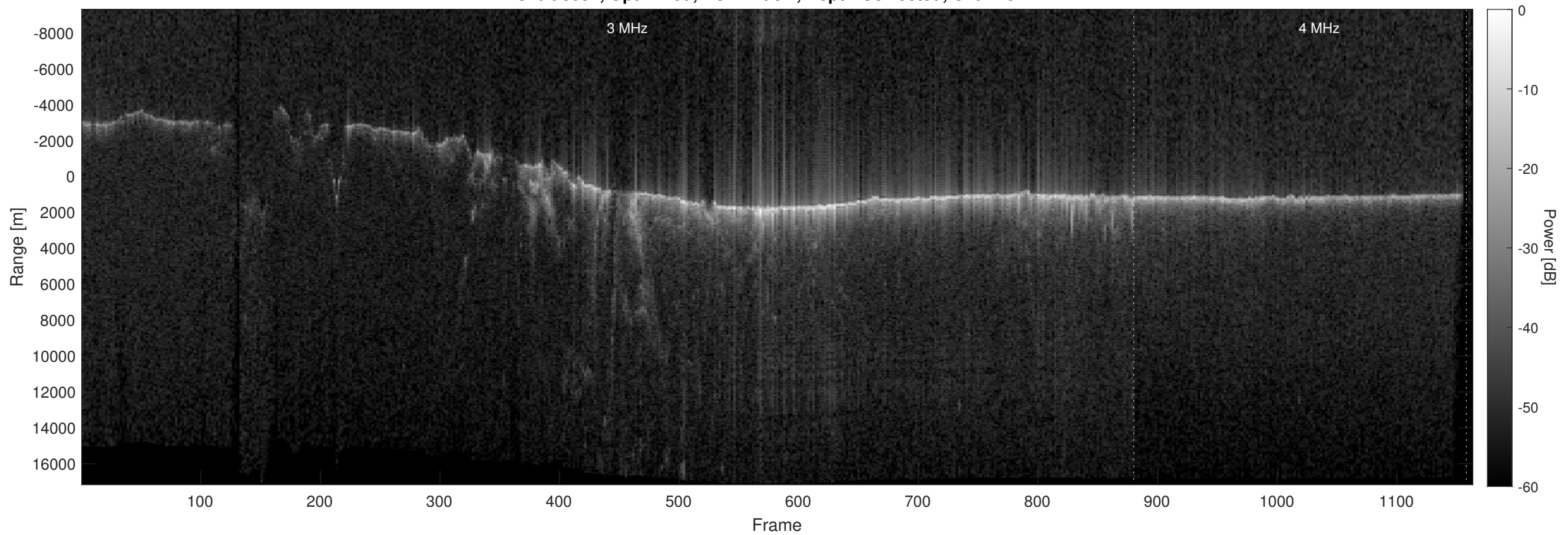
Orbit 8082, Optimized, No Window, Depth-Corrected, Channel 2
