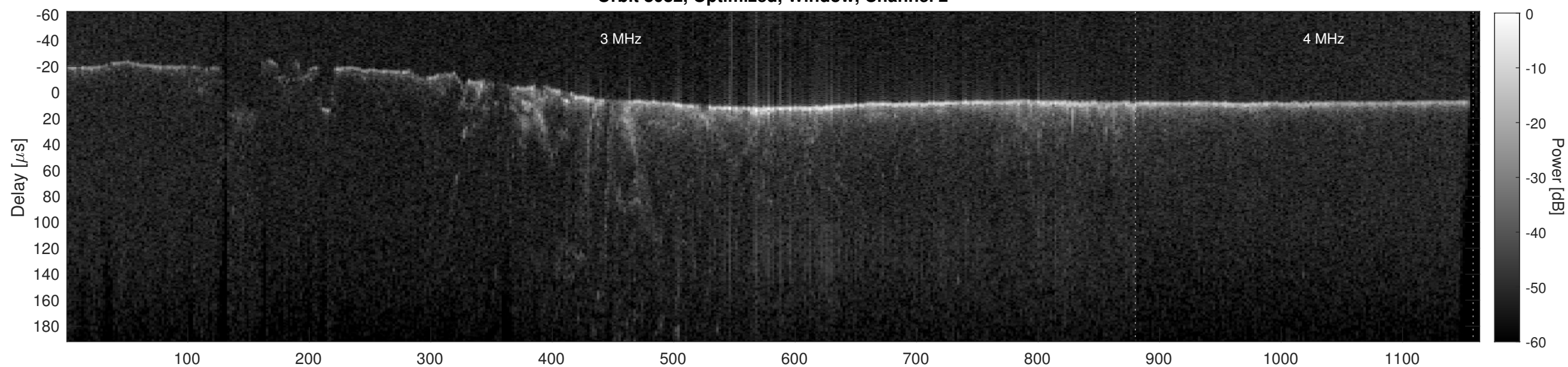
Orbit 8082, Cluttergram
