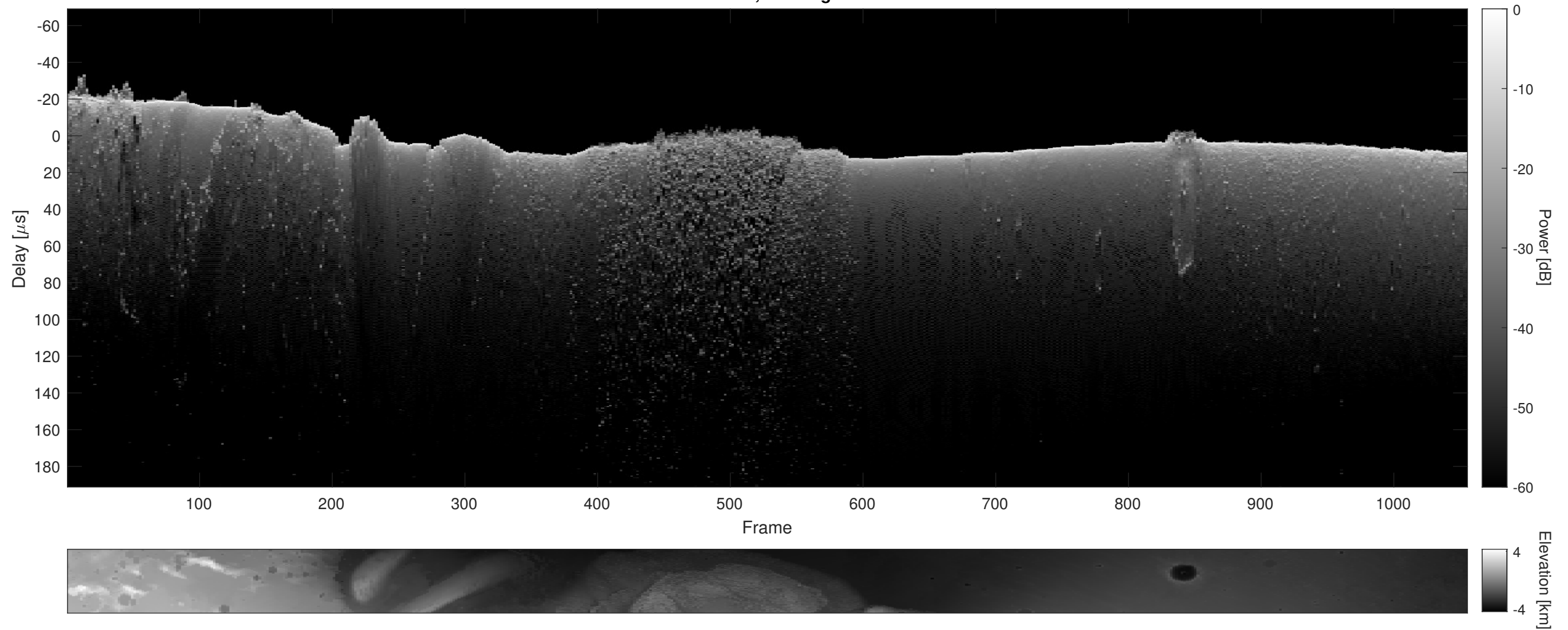
Orbit 8083, Cluttergram
