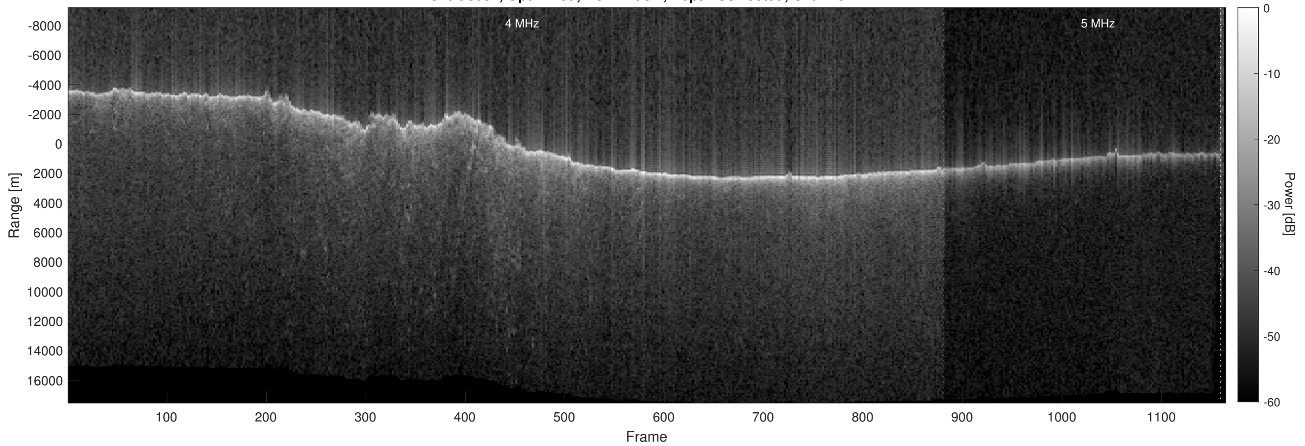
Orbit 8084, Optimized, No Window, Depth-Corrected, Channel 2
