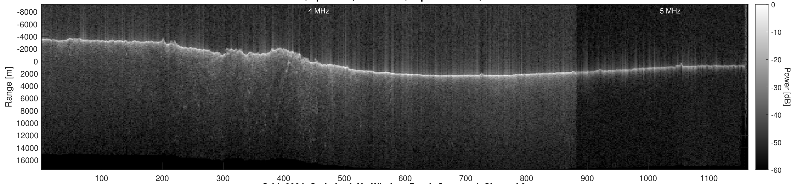
Orbit 8084, Optimized, No Window, Depth-Corrected, Channel 2
