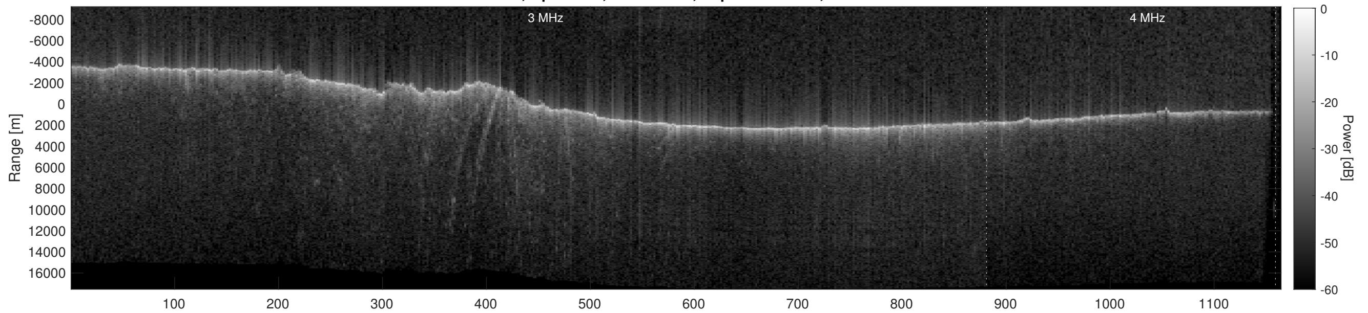
Orbit 8084, Depth-Corrected Cluttergram
