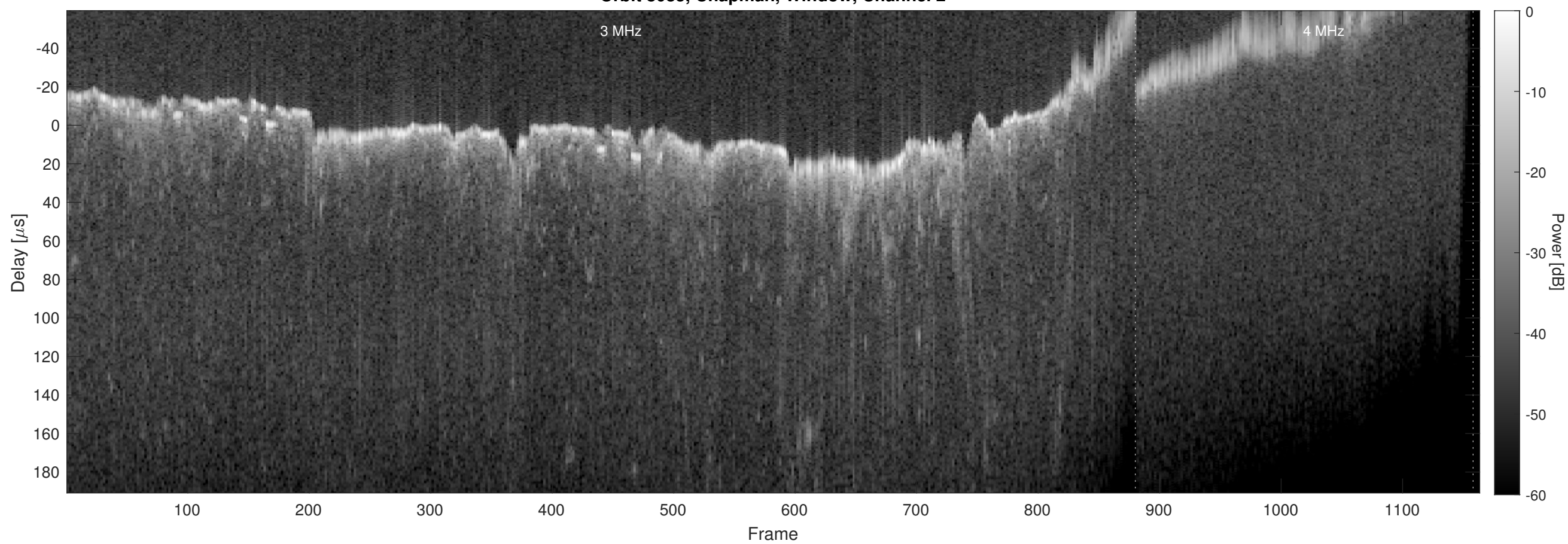
Orbit 8085, Chapman, Window, Channel 2
