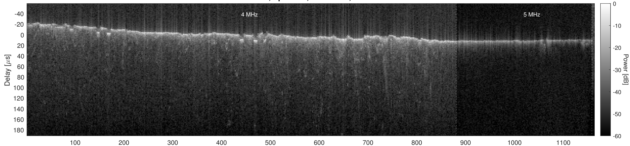
Orbit 8085, Optimized, No Window, Channel 2
