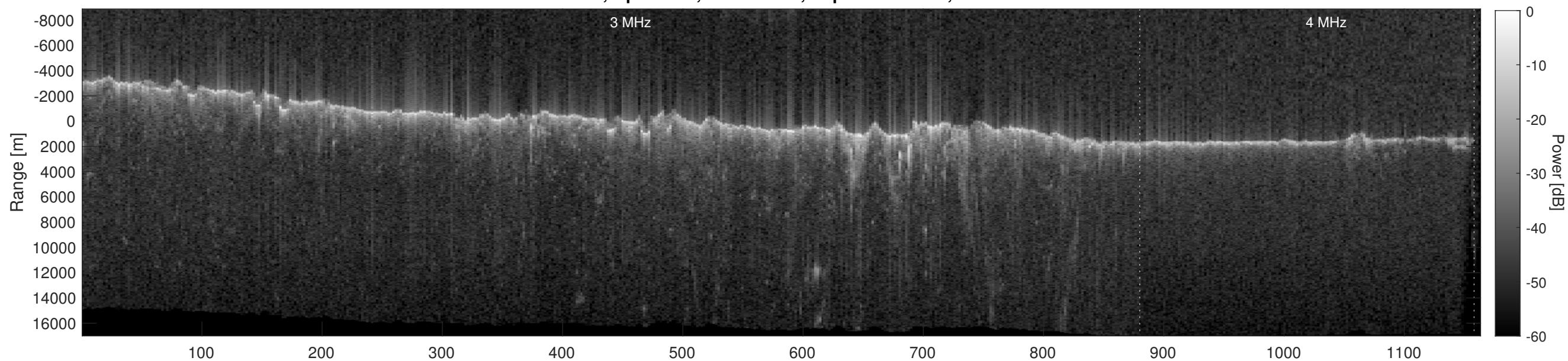
Orbit 8085, Depth-Corrected Cluttergram
