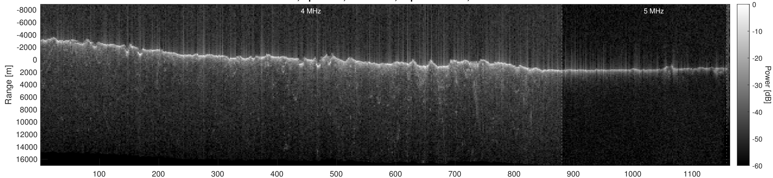
Orbit 8085, Optimized, No Window, Depth-Corrected, Channel 2
