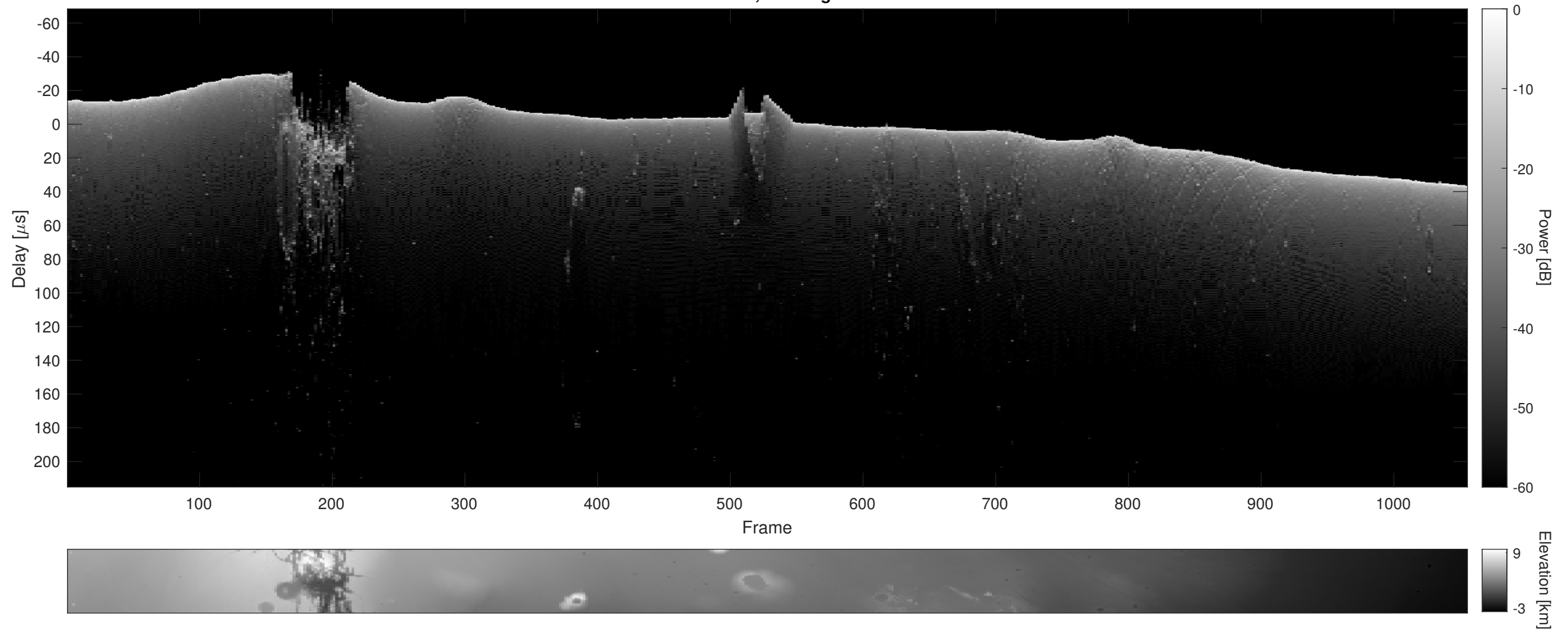
Orbit 8086, Cluttergram
