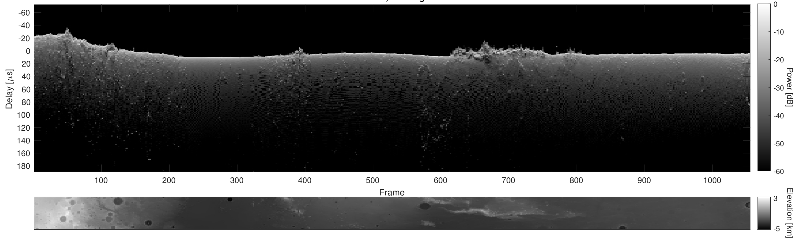
Orbit 8087, Cluttergram
