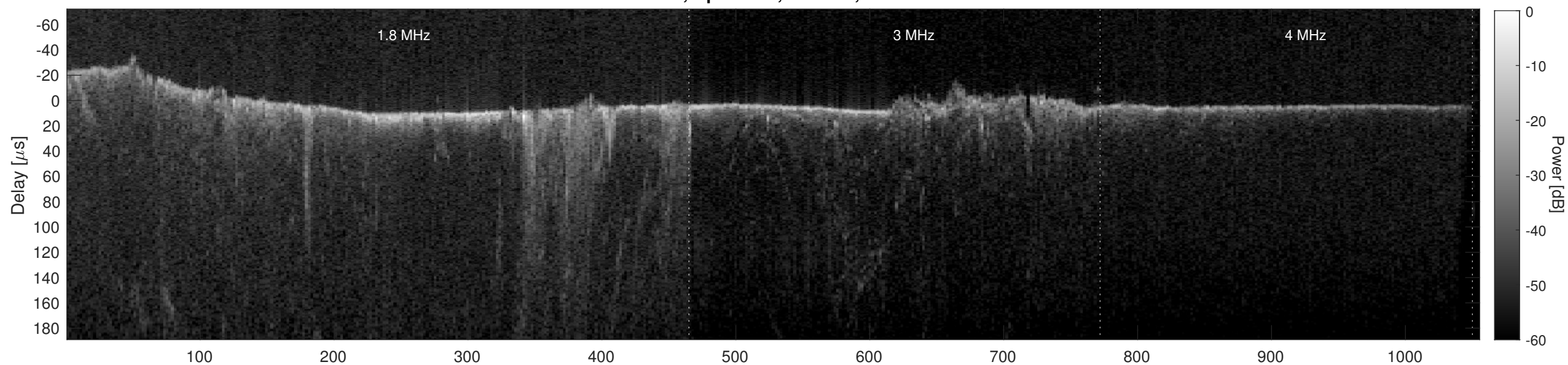
Orbit 8087, Cluttergram
