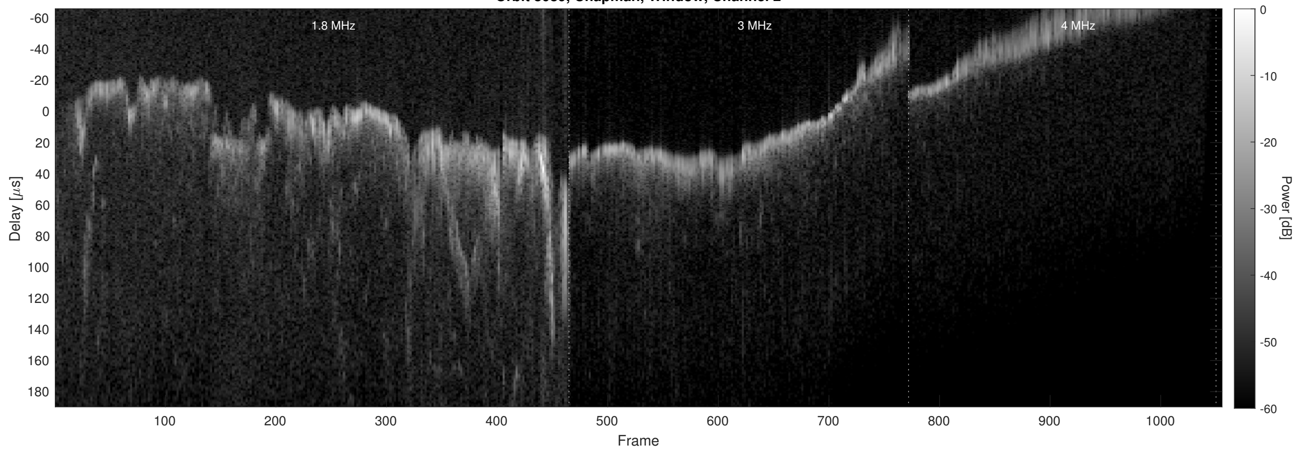
Orbit 8089, Chapman, Window, Channel 2
