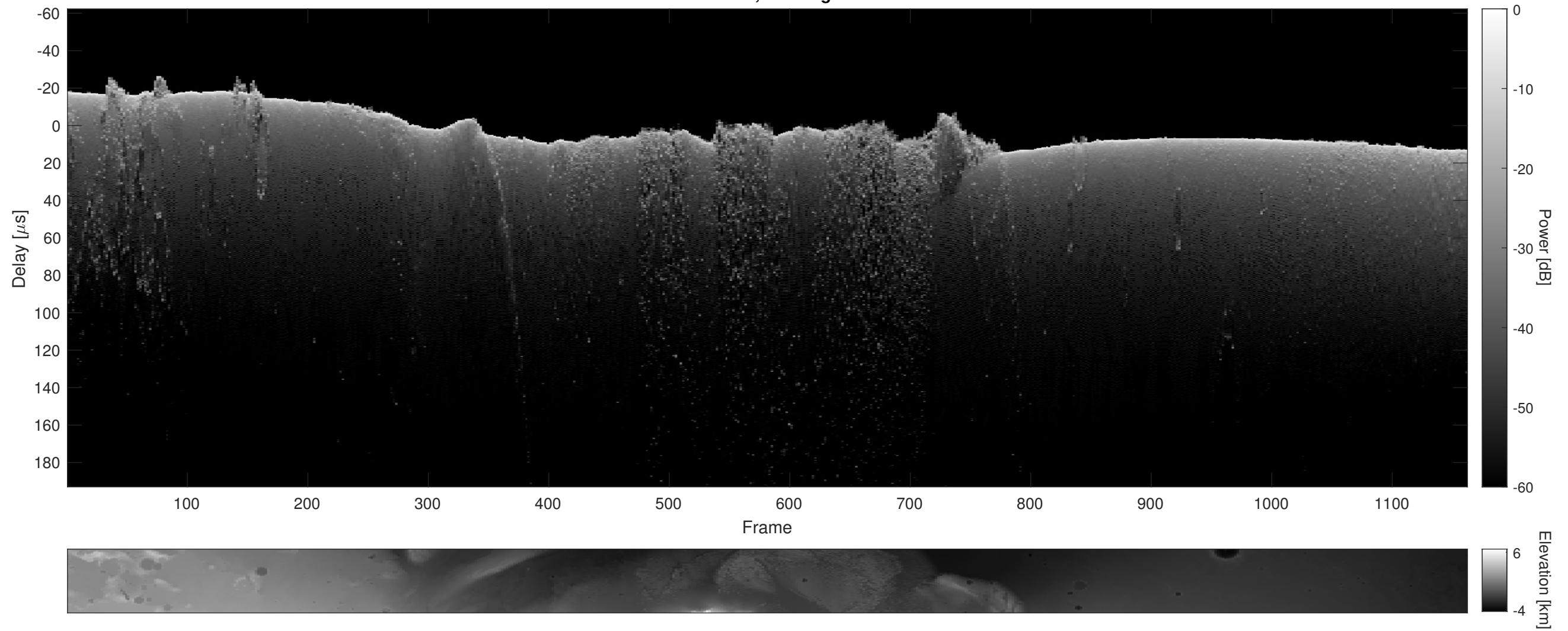
Orbit 8090, Cluttergram
